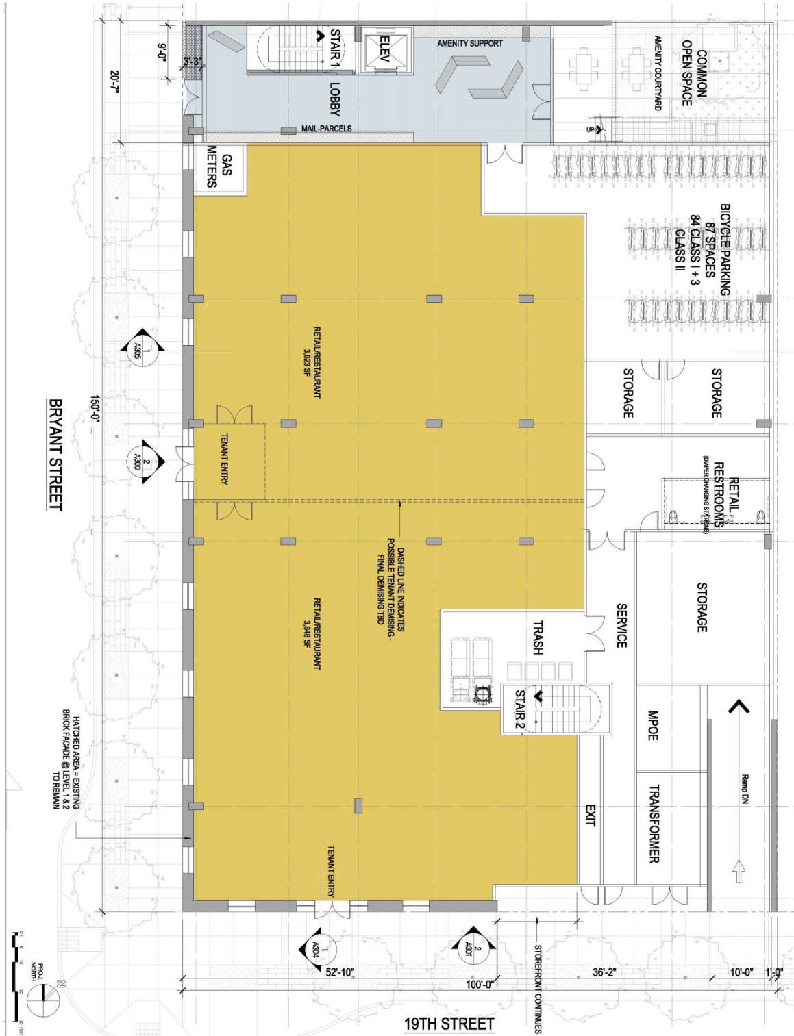
FIGURE 3: PROPOSED GROUND FLOOR
